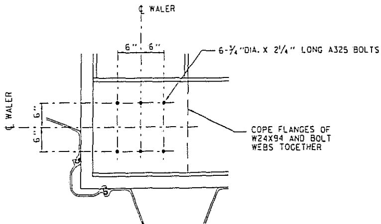
TYPICAL BOLTED CONNECTION AT WALERS
